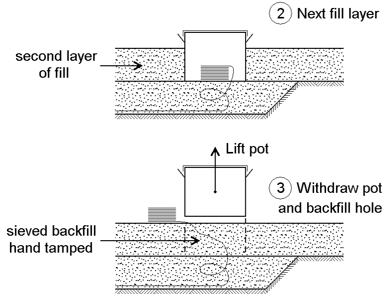
Figure 6: Procedure to route vertically cables (continued)
