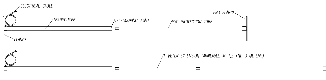
Figure 1: Model ERI fill extensometer
