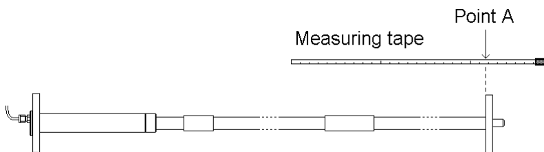
Figure 3a: First step to control the calibration
