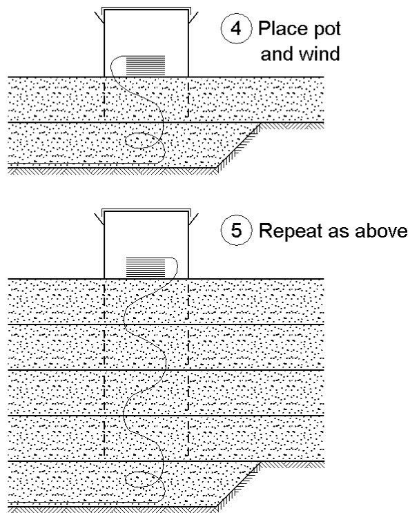
Figure 6: Procedure to route vertically cables
