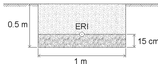
Figure 4: Draft of a trench
